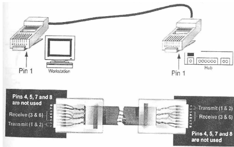
Gambar 13. Kabel Lurus (Straight Cable)
