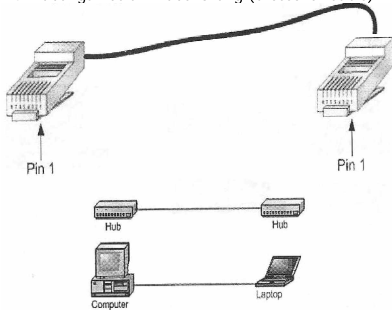
Gambar 15. Kabel Silang (Crossover Cable )
